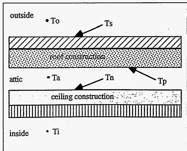
Figure 1. Designation of surface temperatures used in equations 1 through 4.
