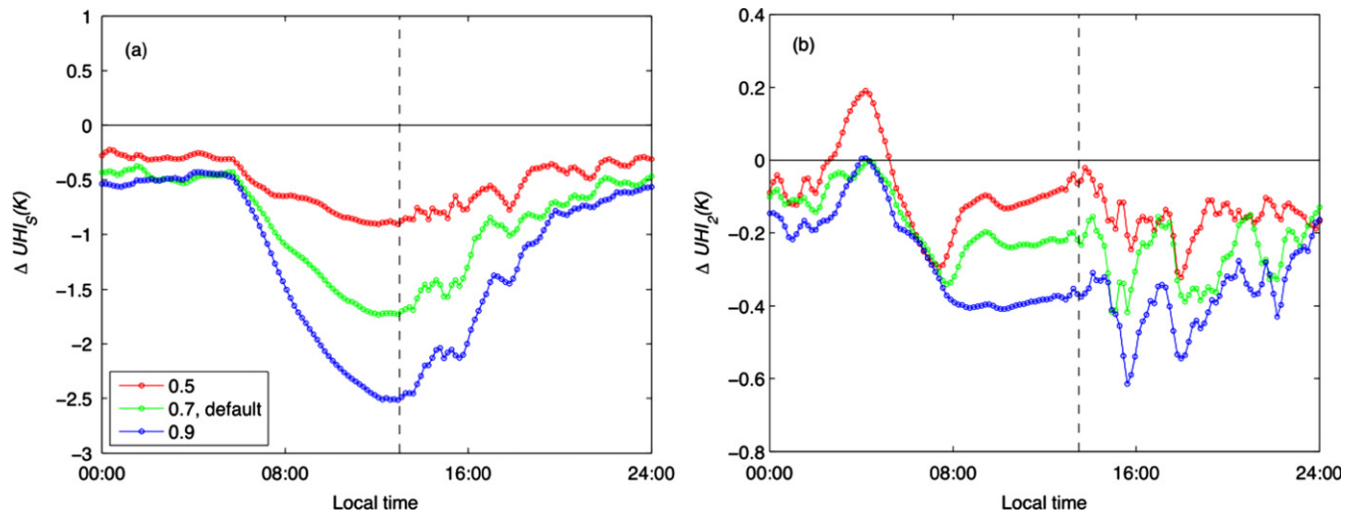
Figure 7. The city-scale impacts of cool roof mitigation strategy as a function of albedo values (the fraction of cool roofs is 50% and the conventional roofs have an albedo value of 0.3): (a) changes in the surface urban heat island and (b) changes in the near-surface urban heat island. The urban heat island effect is the difference in the urban and rural temperatures averaged over domain 3 (water surfaces excluded). All results are averaged over 7 June–10 June. The vertical dashed lines in (a) and (b) indicate when the surface and near-surface temperatures reach their maxima, respectively.
