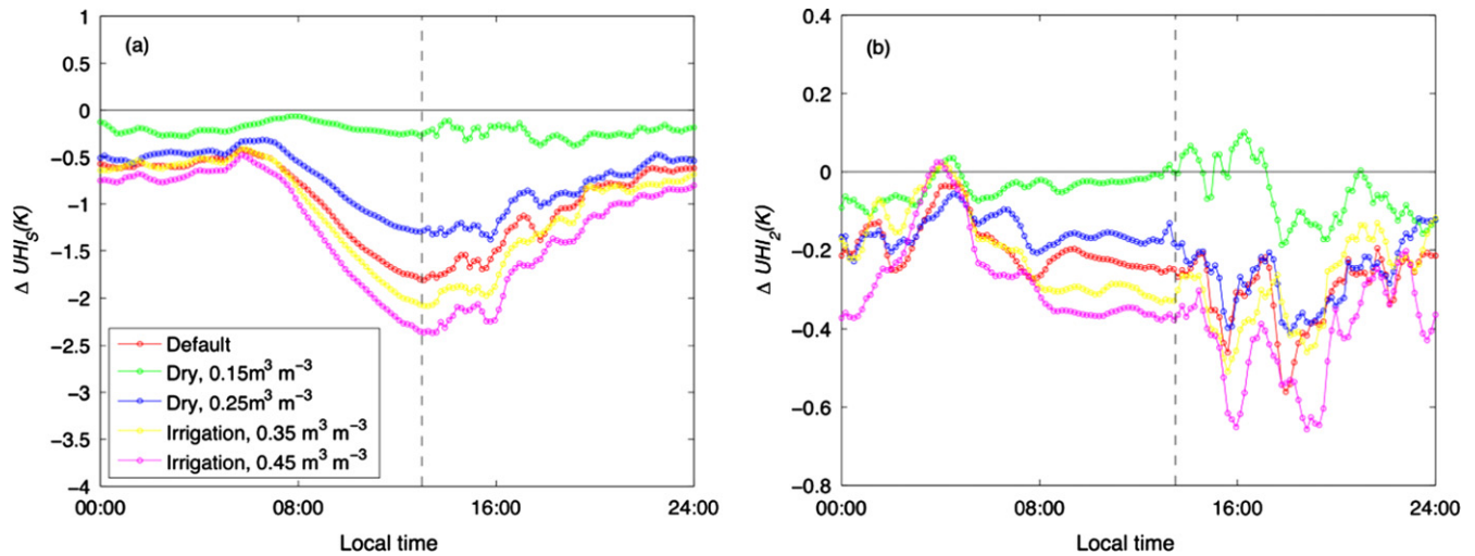
Figure 6. The city-scale impacts of green roof mitigation strategy as a function of green roof soil moisture (the fraction of green roof is 50%): (a) changes in the surface urban heat island and (b) changes in the near-surface urban heat island. The urban heat island effect is the difference in the urban and rural temperatures averaged over domain 3 (water surfaces excluded). All results are averaged over 7 June–10 June. The vertical dashed lines in (a) and (b) indicate when the surface and near-surface temperatures reach their maxima, respectively.
